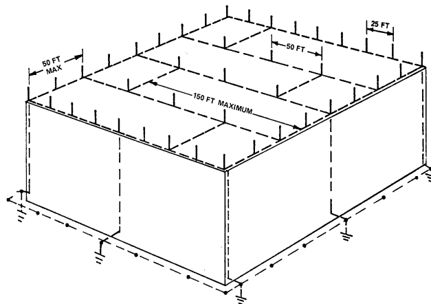
Diagram: Air Terminal, Conductor, and Down Conductor Spacing for an LPS
